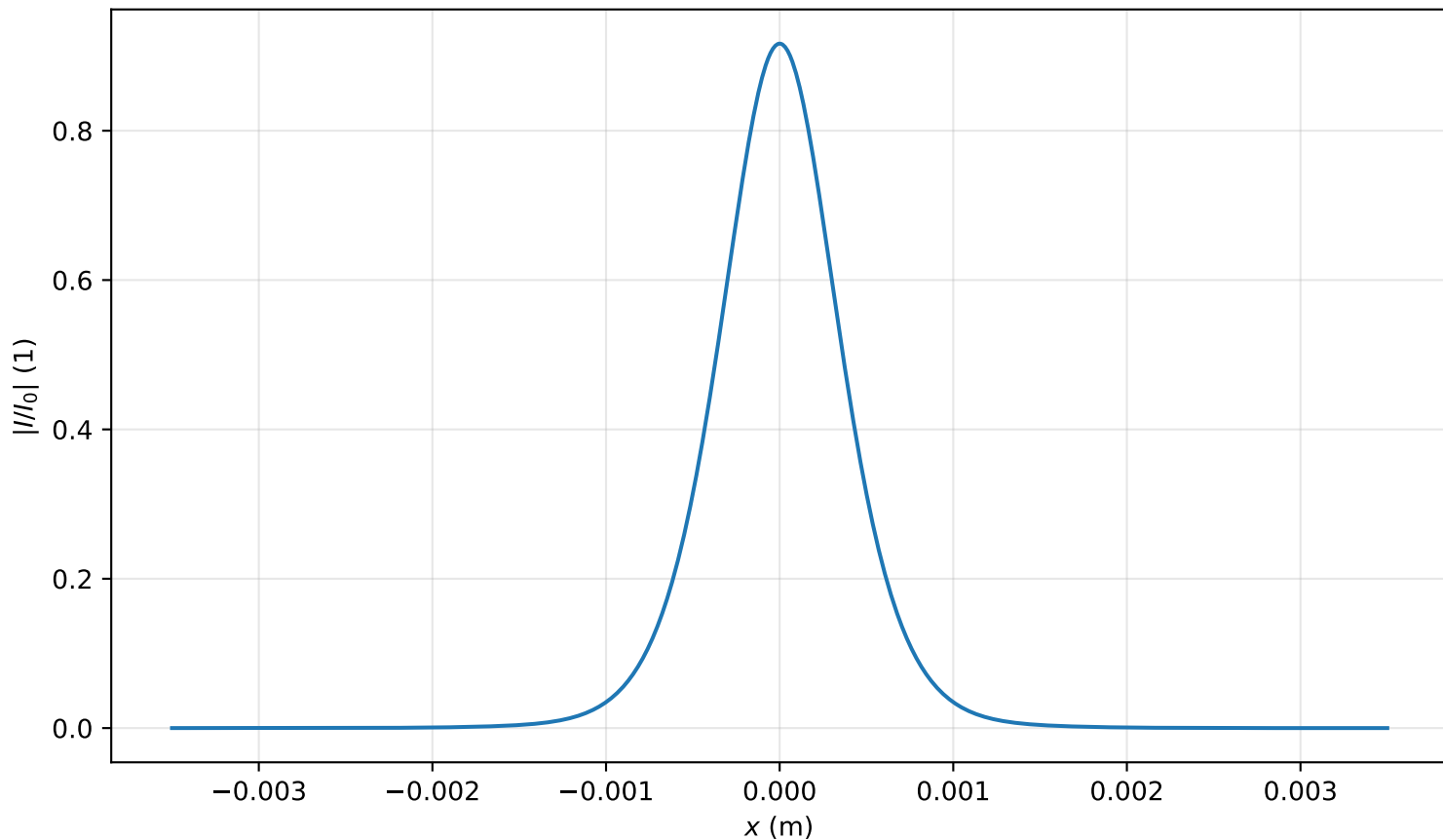
Intensity profile I(x, y = 0, z = 2.707m)/I_0 , P_{in}=0.7P_{cr} , artificial time
